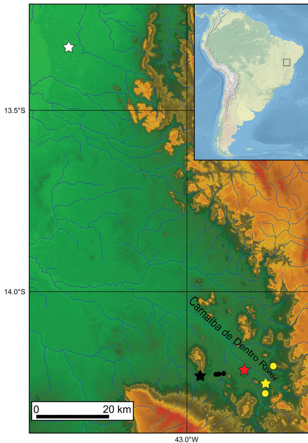
Figure 4. Geographical distribution of species of the Hypsolebias J'-clade in the upper Carnaíba de Dentro River drainage (yellow, H. fulminantis ; red, H. splendissimus ; black, H. carlettoi and H. shibattai (white); stars indicate type localities.
