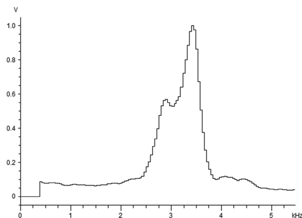
Figure 17. Power spectrum of an advertisement call from Choerophryne bisyllaba sp. n.
